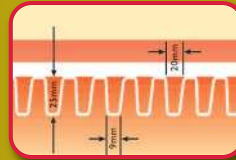
← Optimum radiant heat created by outer High Fin Surface area
